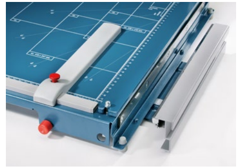
Pull-out front stop up to 170 mm with fold-out paper holders for cutting strips of equal width
